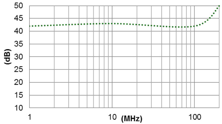
Reverse Isolation
