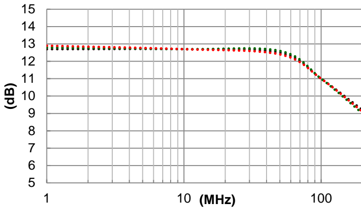
Gain
